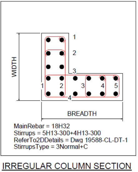
S4 – Fig 23 : Irregular Column Section
