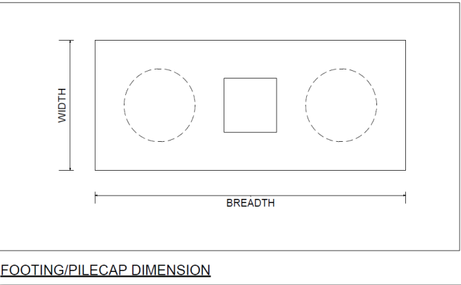
S4 – Fig 47: Dimension Definitions for Footing / Pilecap
