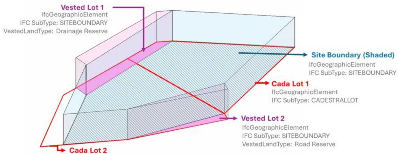
S4 – Fig 113 : Illustration for modelling Site Boundary and Cadastral Lot
