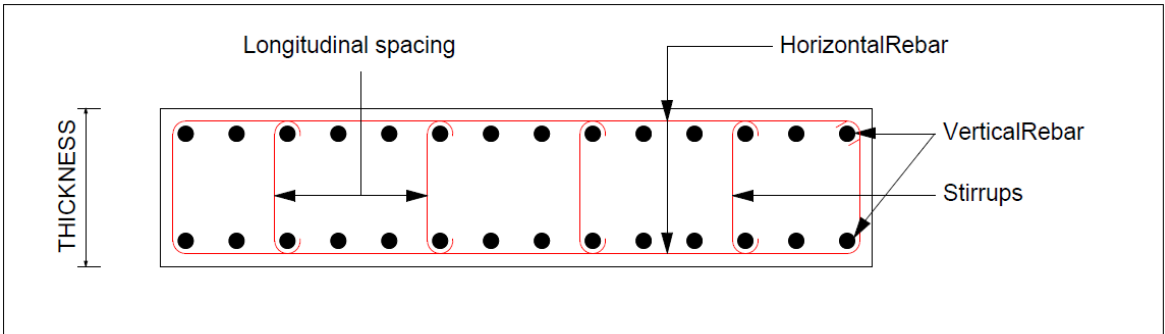
S4 – Fig 142 : Wall Reinforcement Annotation
