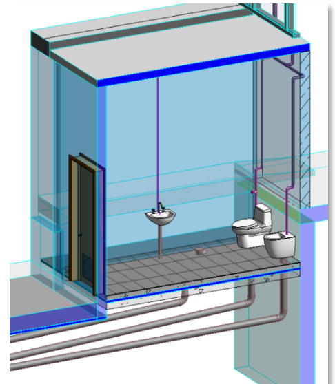
S4 – Fig 108 : Water Closet
