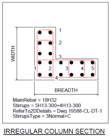
S4 – Fig 37: Irregular Column Section
