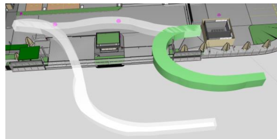
S4 – Fig 97: Refuse Truck Swept Path (Egress)
