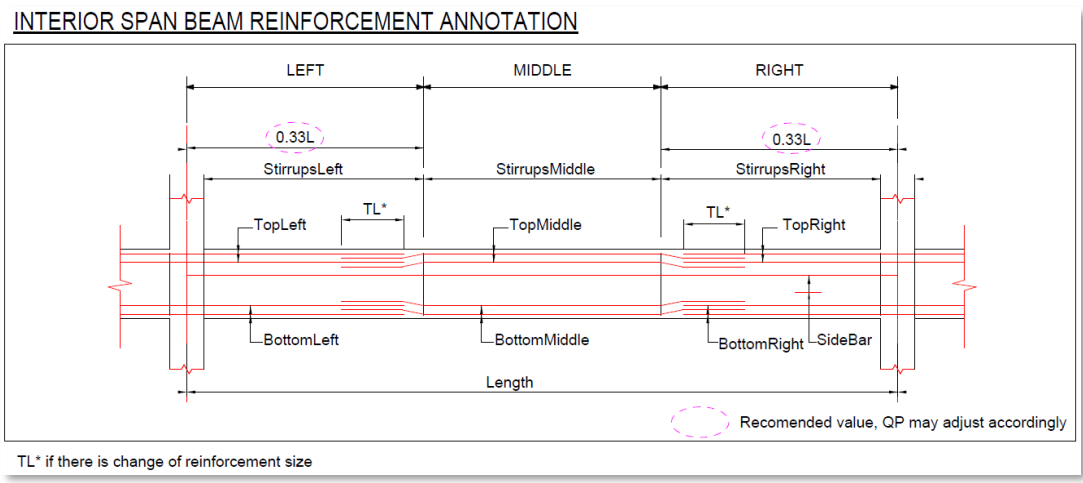
S4 – Fig 21: Beam Annotation Interior Span
