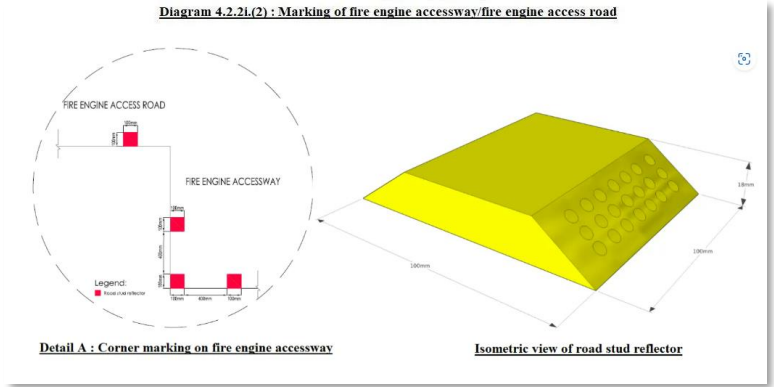
S4 – Fig 101 : Marking of Fire Engine Accessway
