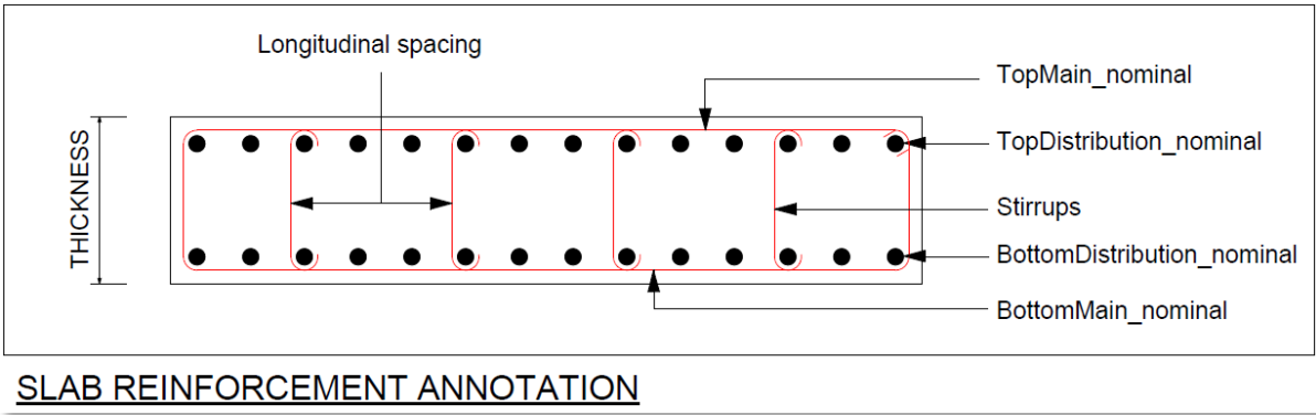
S4 – Fig 117 : Slab Reinforcement Annotation
