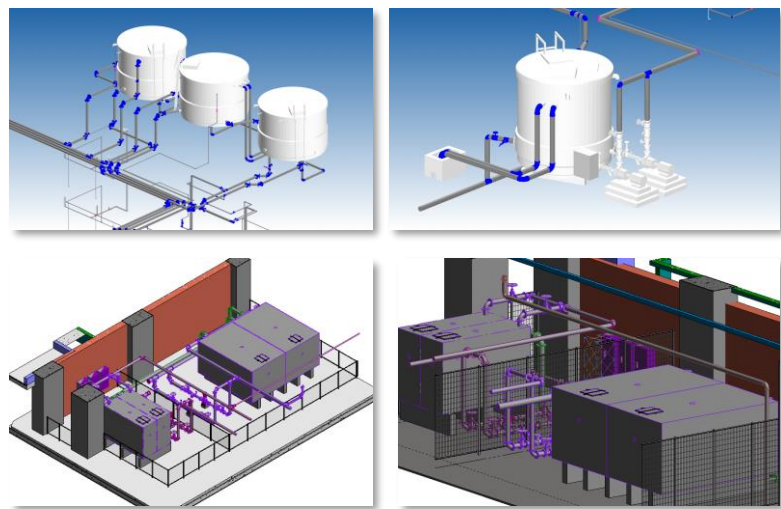
S4 – Fig 138 : Water Tank
