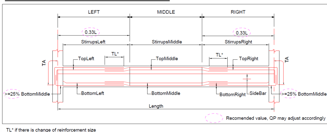
S4 – Fig 19: Beam Annotation Single Span
