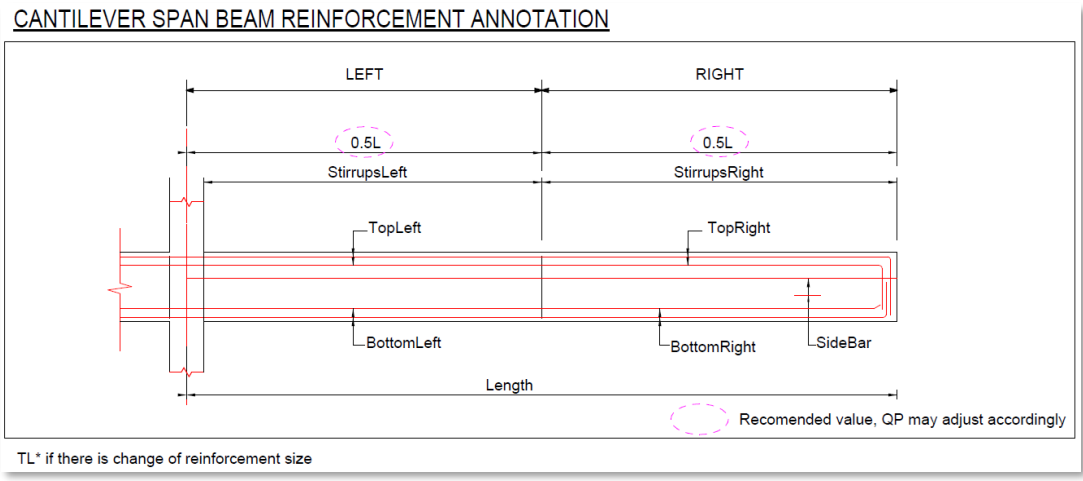
S4 – Fig 22: Beam Annotation Cantilever Span
