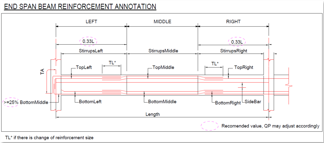
S4 – Fig 20: Beam Annotation End Span
