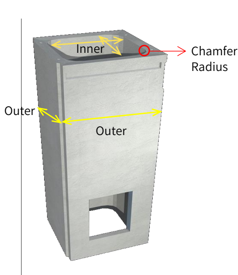
S4 – Fig 93 : Singular Refuse Chute
