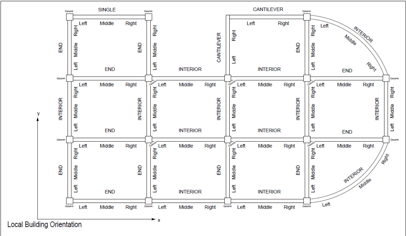
S4 – Fig 18: Beam Sequencing and Span Definition
