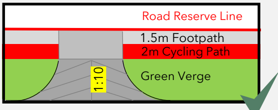
Figure 1.4 - Example of Vehicular Access where Gradient of Entrance Approach Stops at the Edge of the Crossing (Accurate)
