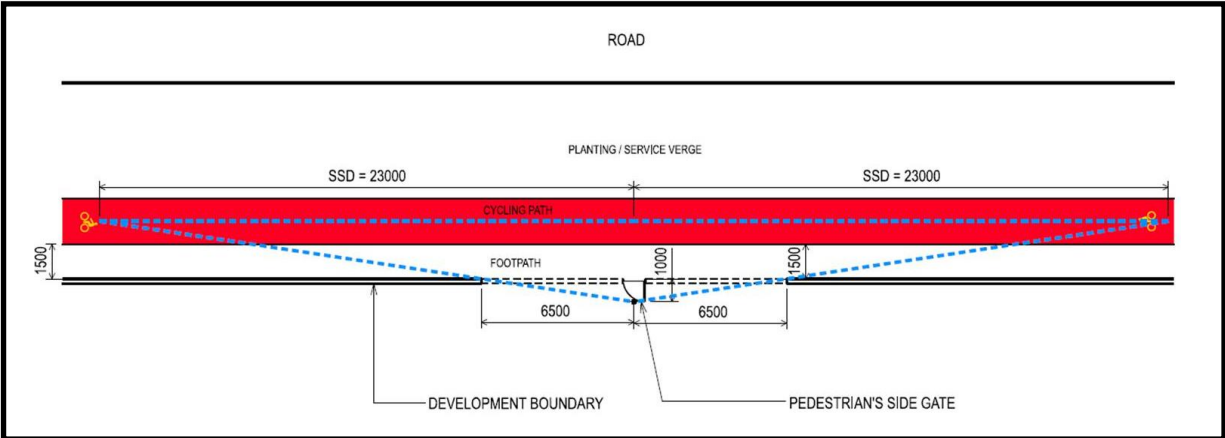
Figure 3.1 - Designing for Clear Line of Sight at Pedestrian Access (Cycling Path)
