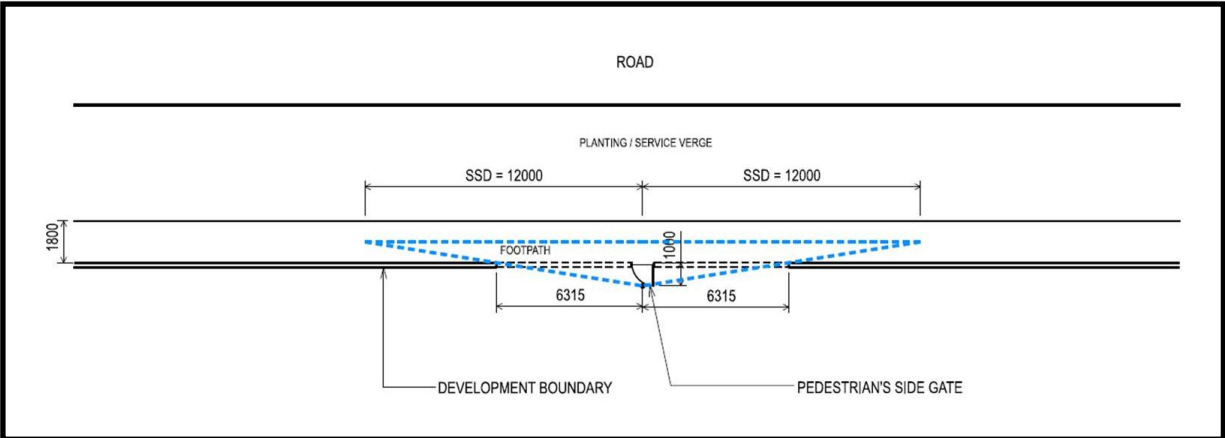
Figure 3.2 - Designing for Clear Line of Sight at Pedestrian Access (Footpath)
