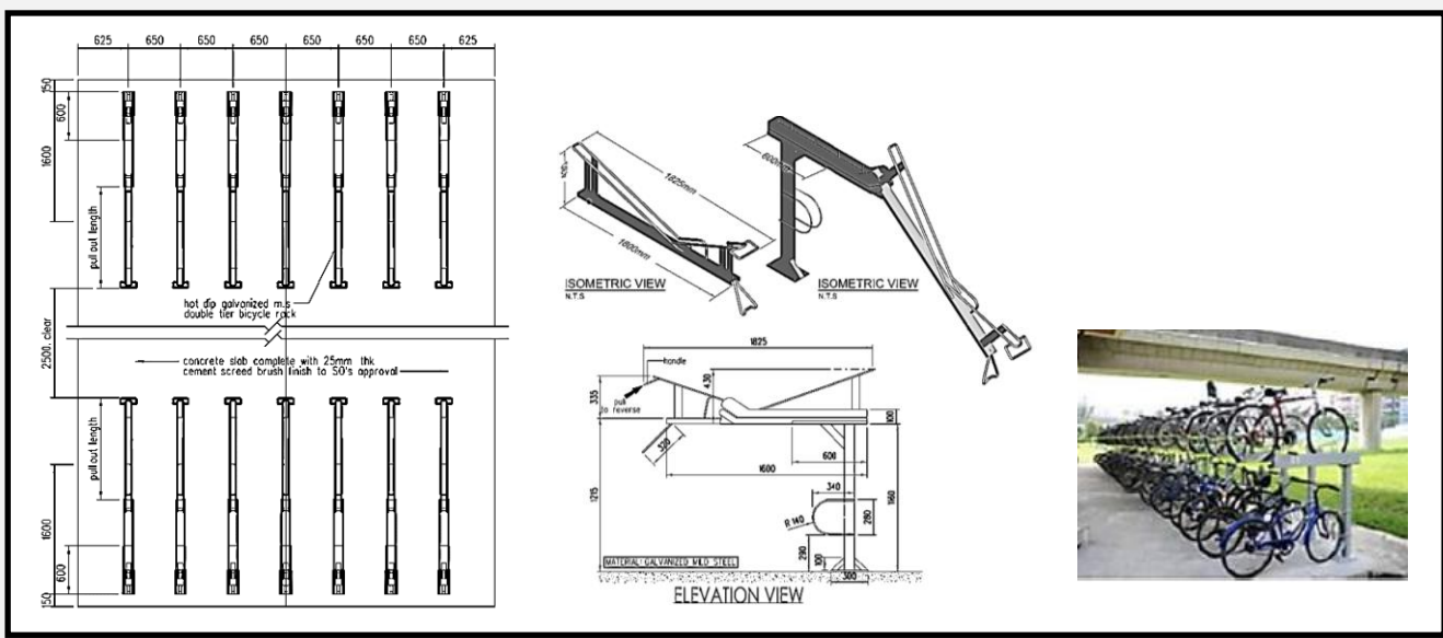
Figure 4.2 - Double Tier Bicycle Parking Details
