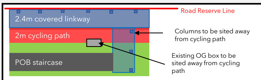
Figure 1.3 - Paths shall be free from encumbrances
